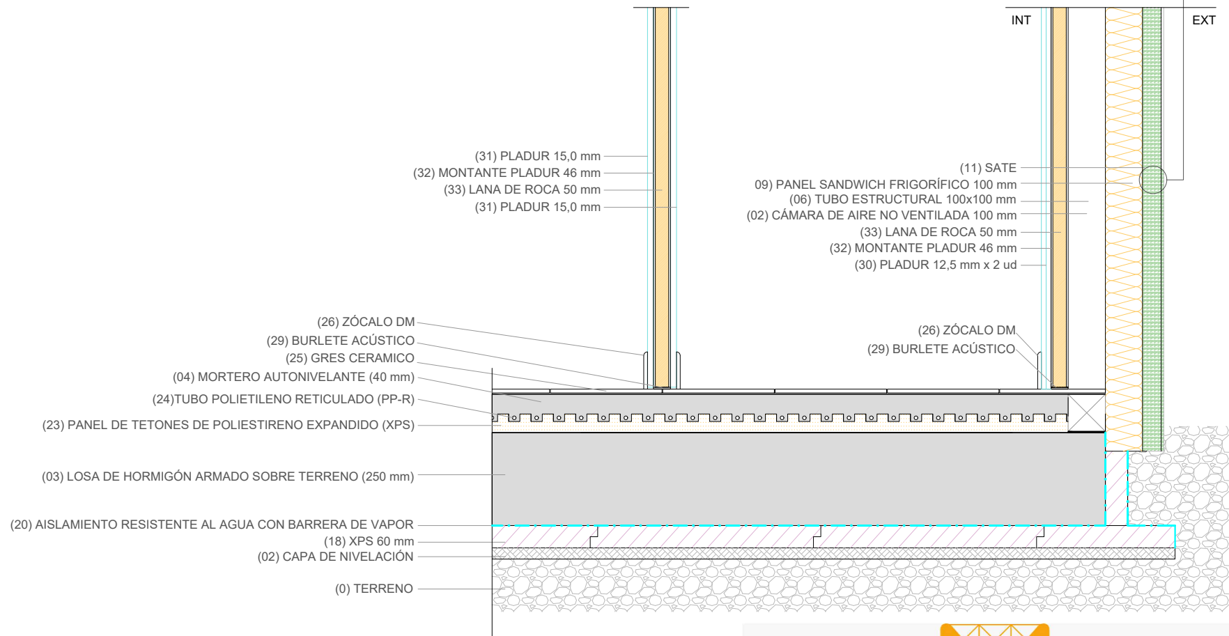
FS1 - Floor slab
