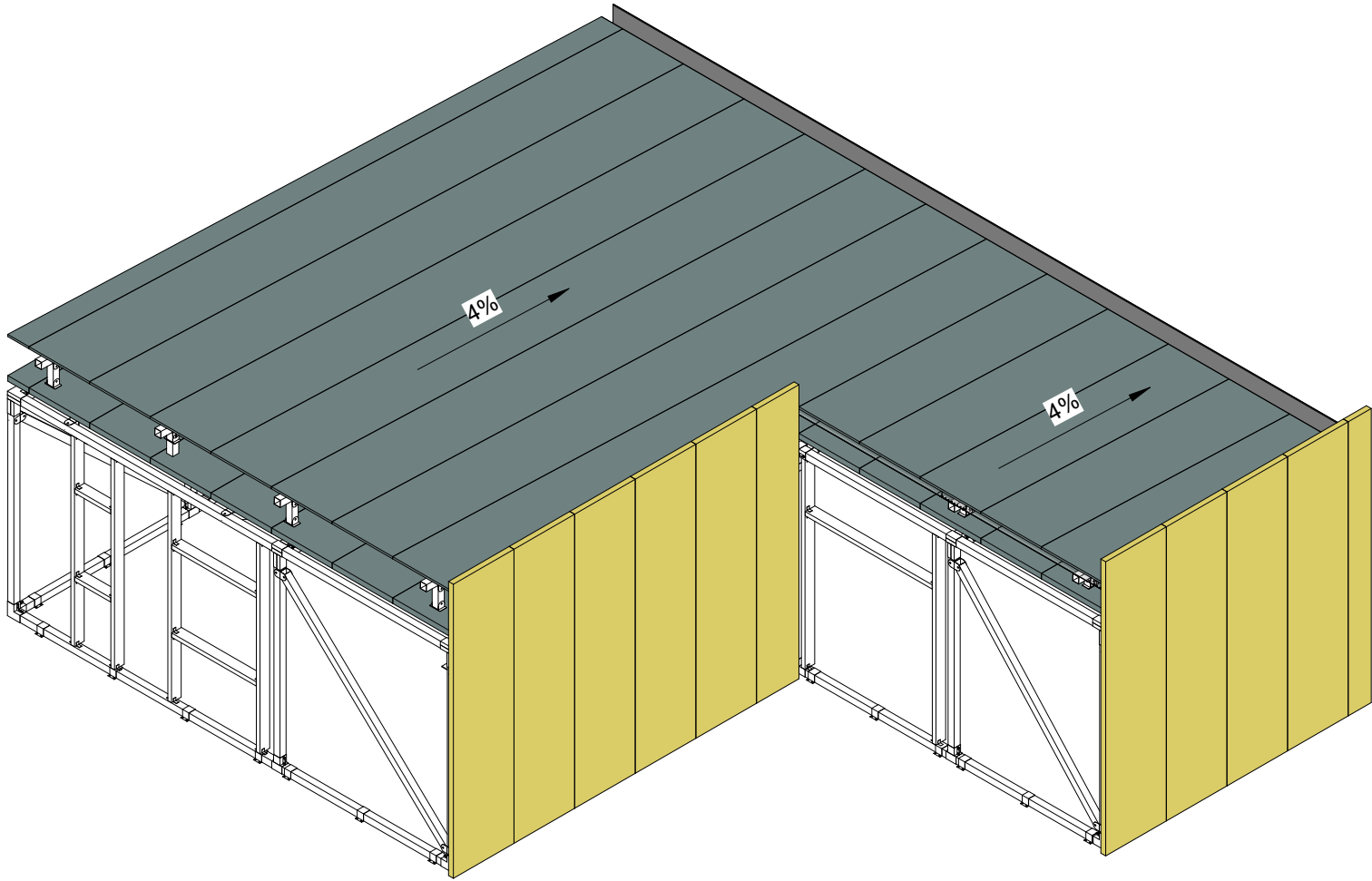
2 3D Fachada 3 P-05
