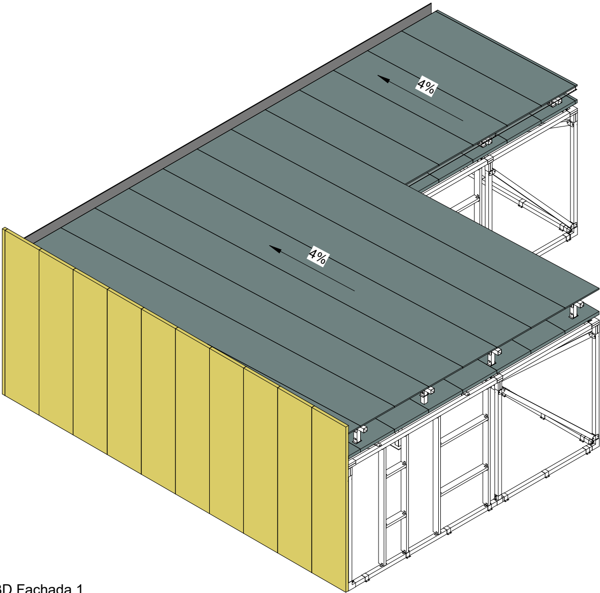
2 3D Fachada 1 P-03
